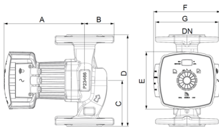
Fig. 3: Flanged pump set
