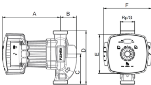
Fig. 2: Screw-ended pump set
