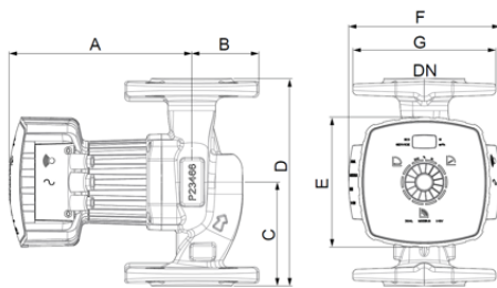
Fig. 3: Flanged pump set
